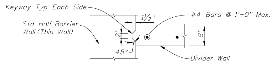
SECTION FF
