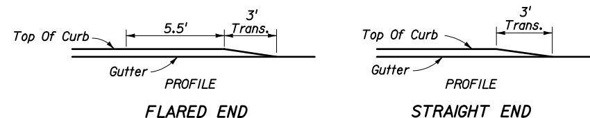
CURB TYPE A
