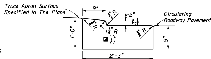
TRAFFIC BEARING SECTION FOR USE IN ROUNDBOAT CENTRAL ISLAND CONSTRUCTION TYPE RA
