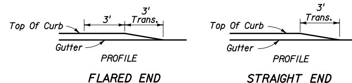
CURB AND GUTTER TYPES E & F
