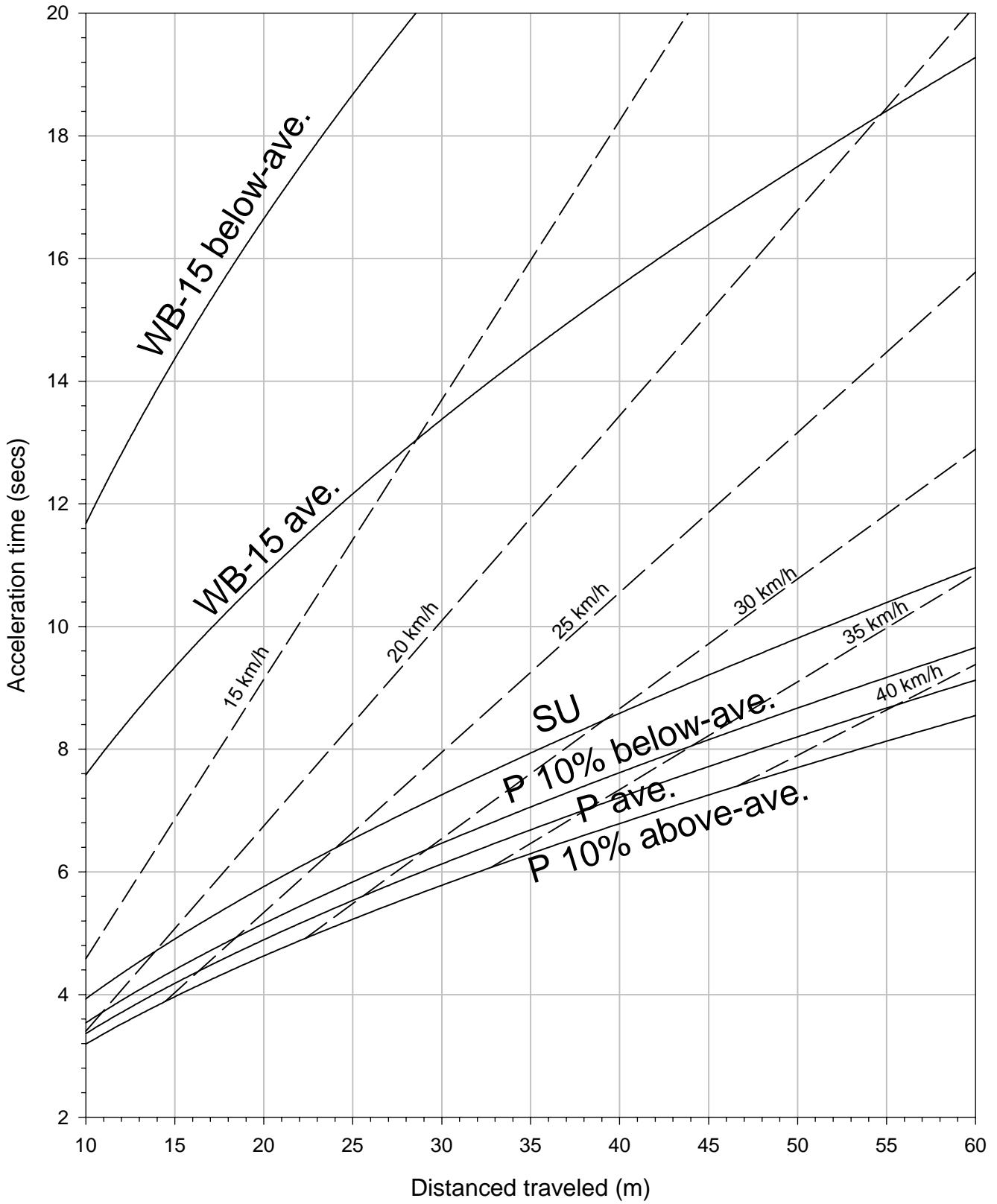
FIGURE 3 Times and Distances from Stop for Recommended Design Accelerations
