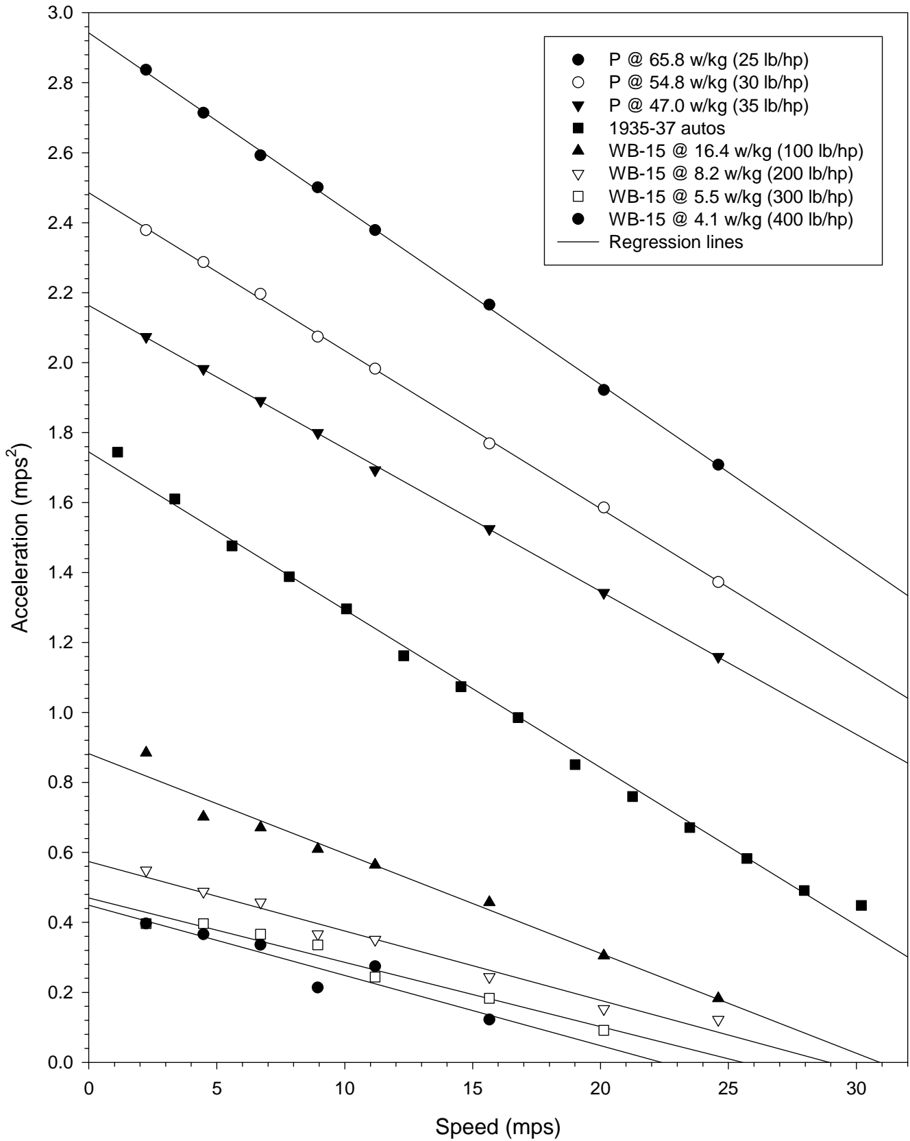
FIGURE 1 Vehicle Maximum Accelerations
