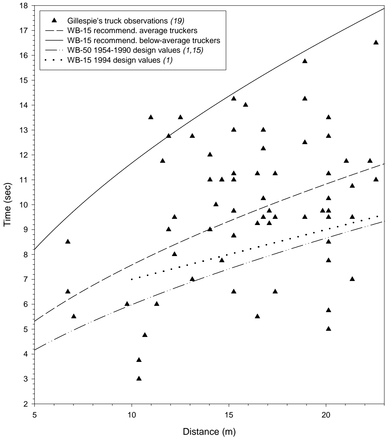
FIGURE 4 Times and Distances from Stop for Heavy Truck Accelerations
