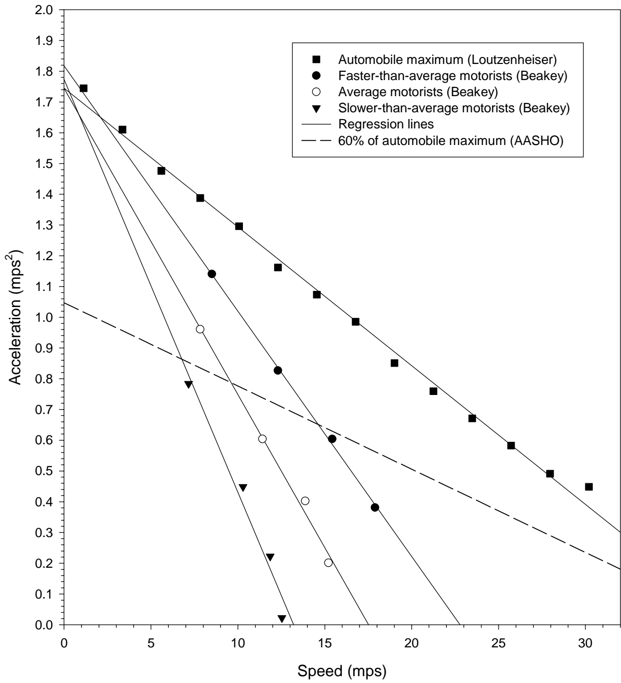
FIGURE 2 Observed 1935-37 Traffic Accelerations
