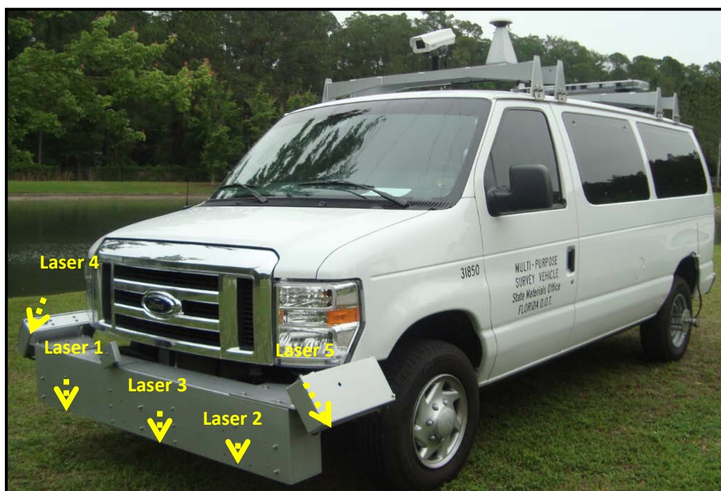
Figure 1. FDOT MPSV with 5 Laser Height Sensors Mounted in the Front Bumper
