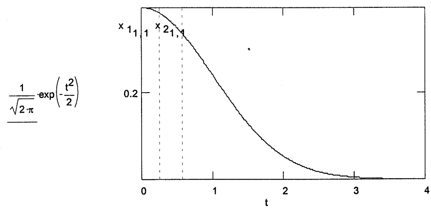
Channel pier impact width location on 'bell curve' for first barge group.
