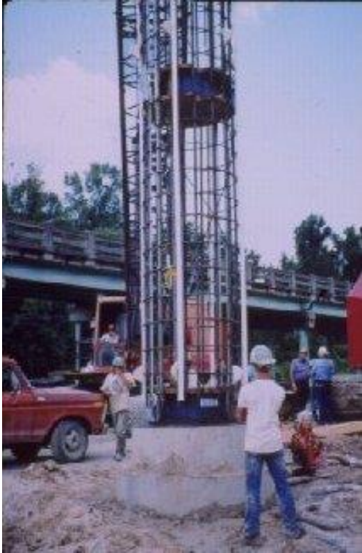
Figure 38, Osterberg Load Cells
