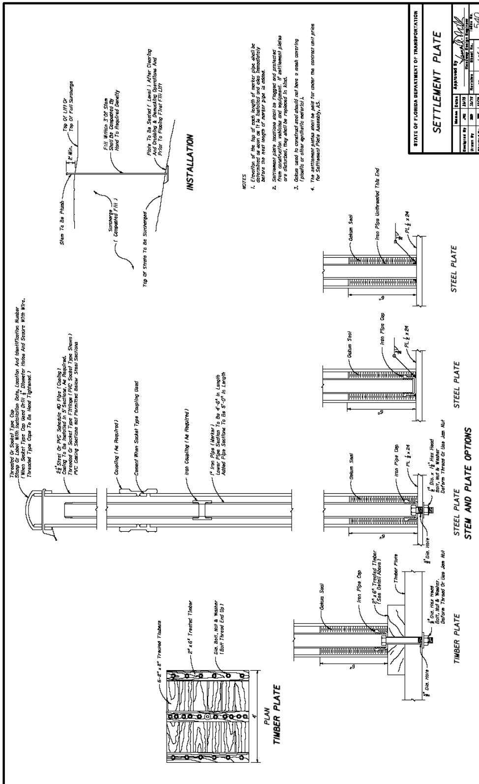
Figure 25, Typical Settlement Platform Design (Standard Plans, Index 141-T01)
