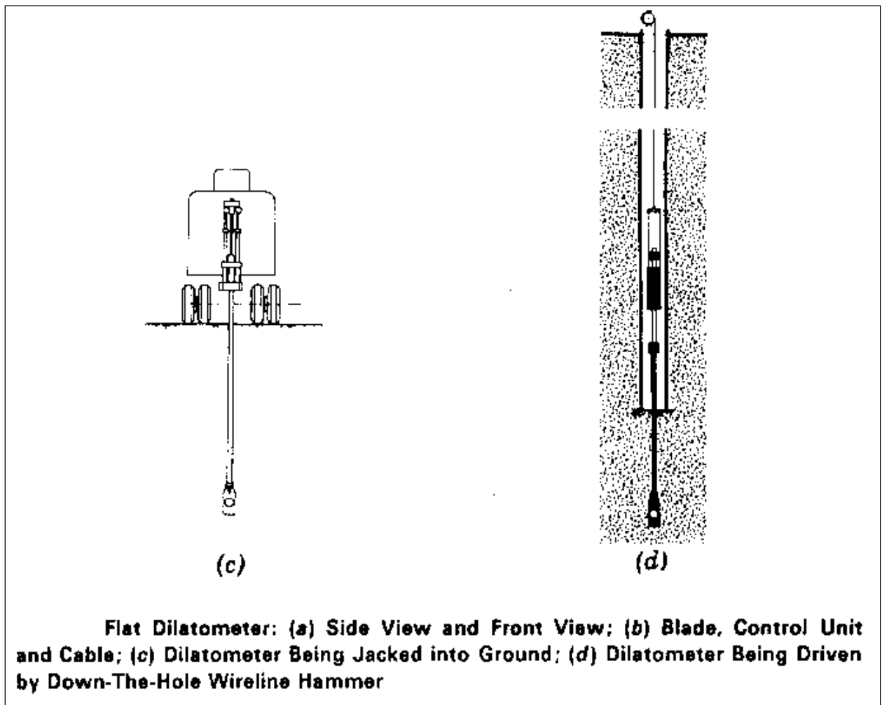
Figure 11, Dilatometer (Continued)
