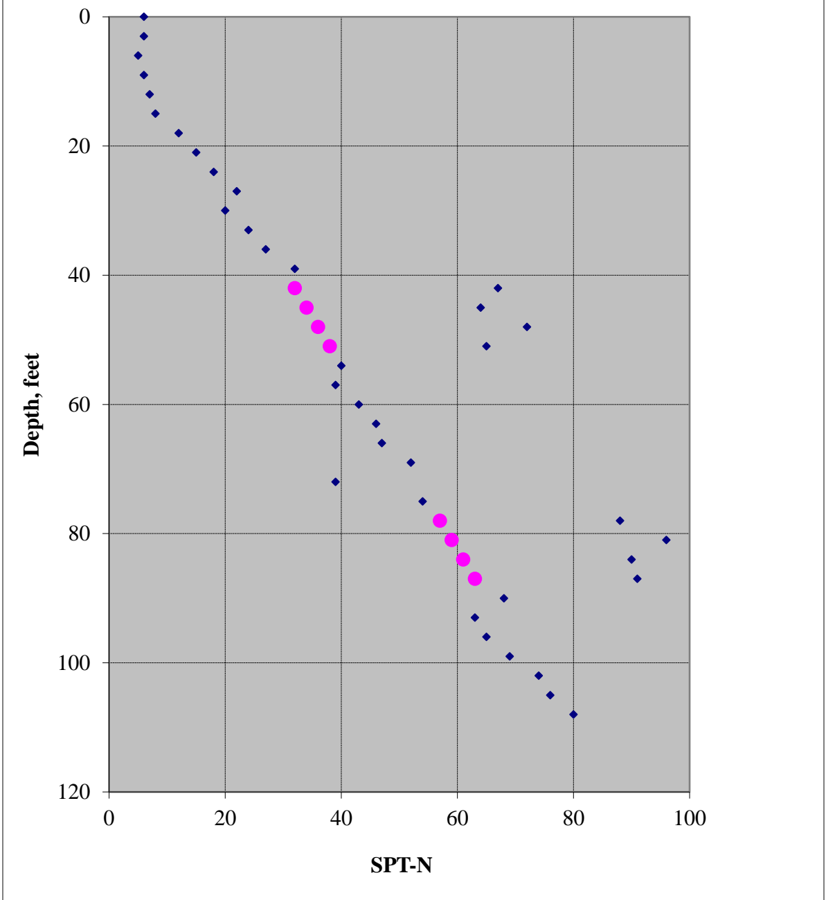
Figure 5, Example SPT-N Adjustments Due to Plugged Sampler
