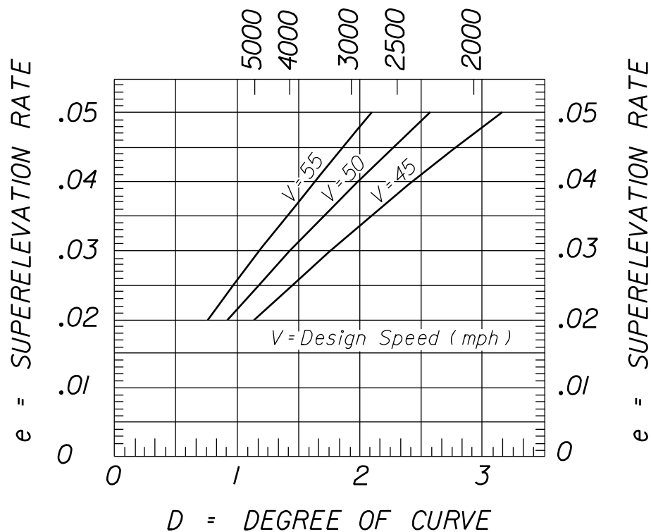
Figure 2.16.3 Superelevation Rates for Suburban Sections R = \text{RADIUS OF CURVE - FEET}
