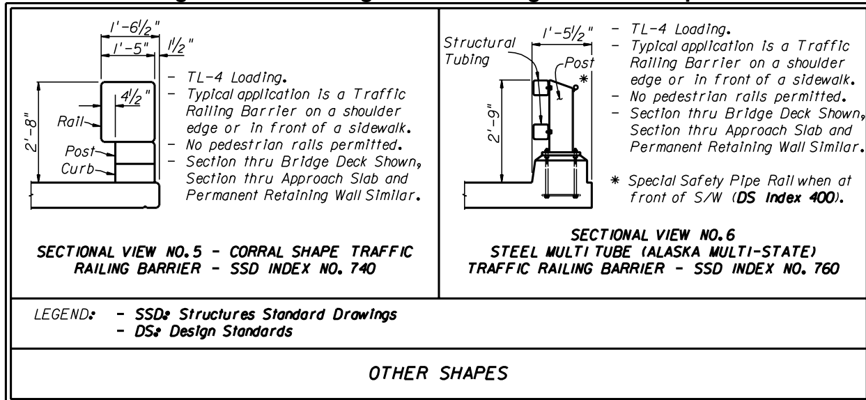
Figure 2.12.2 Bridge Traffic Railings – Other Shapes
