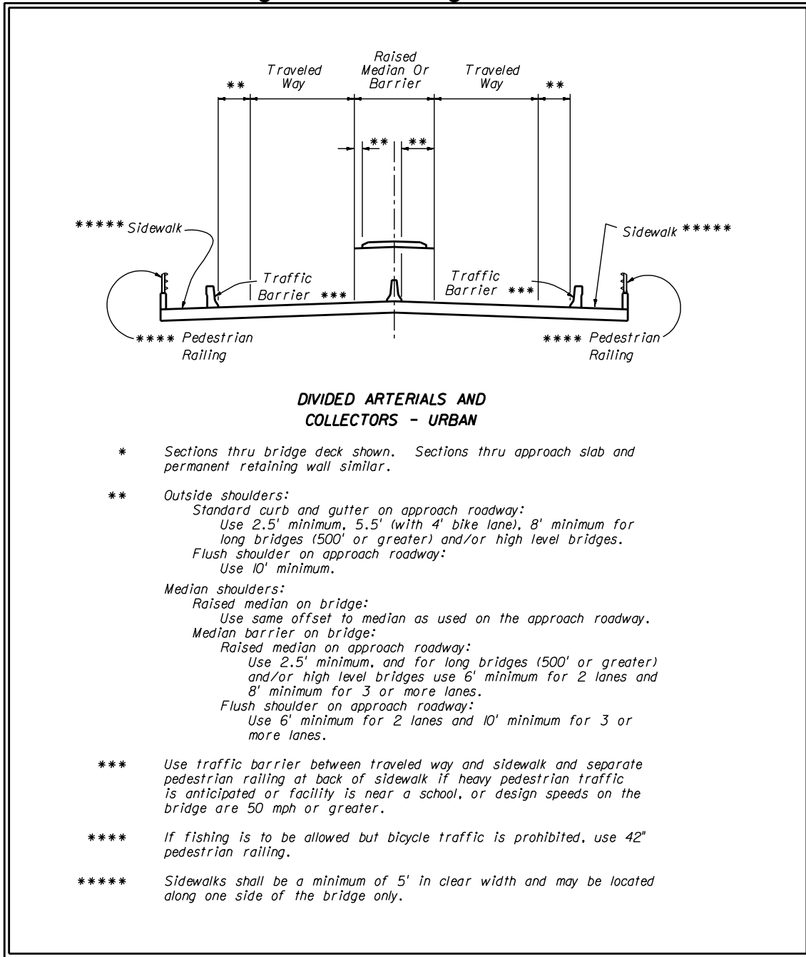
Figure 2.0.4 Bridge Section *
