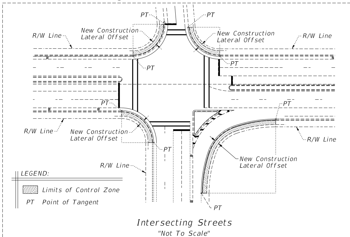
Figure 4.2.4 Intersection Radii
