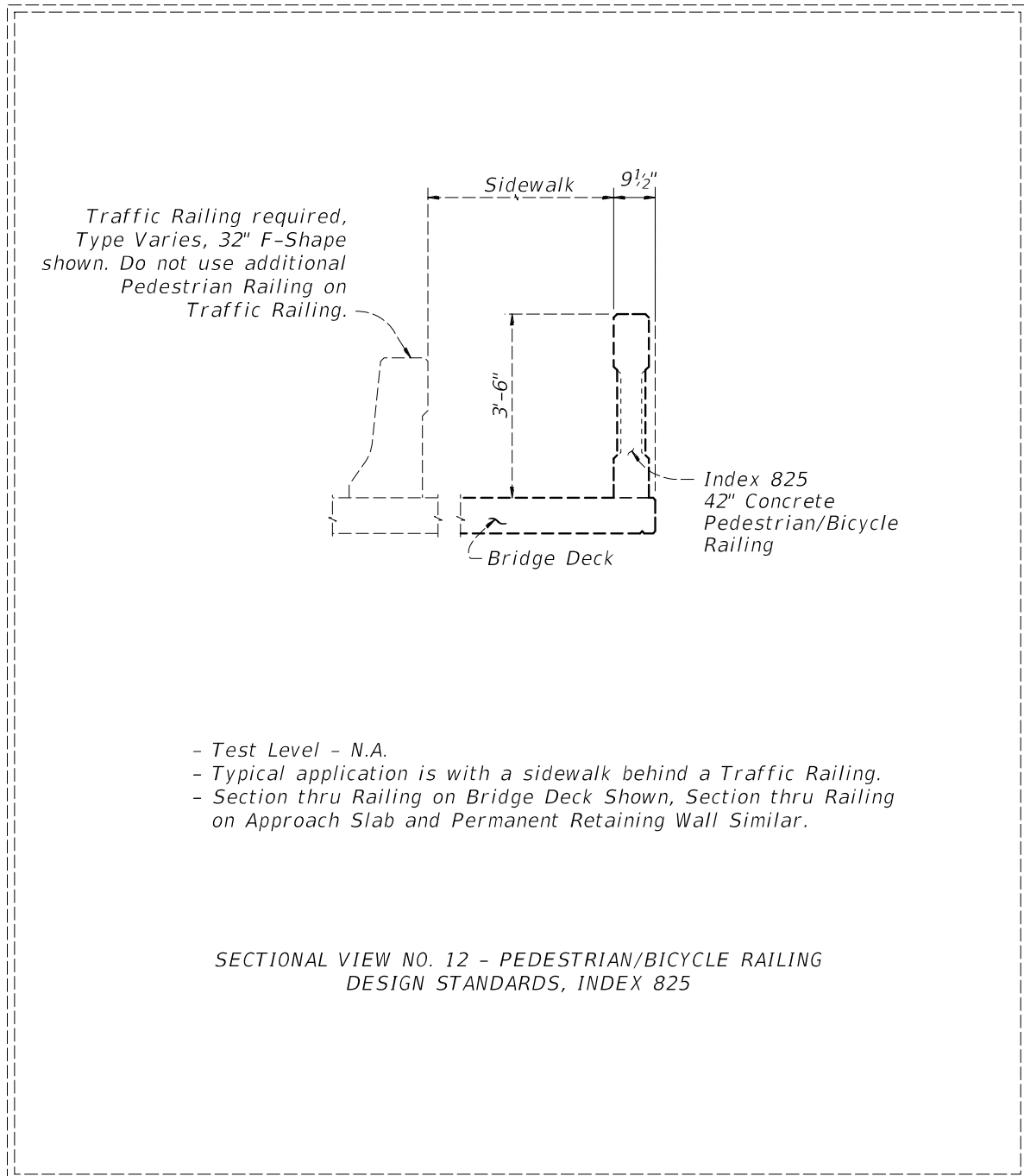
Figure 4.4.7 Bridge Railing – Pedestrian/Bicycle Railing (Index 825)
