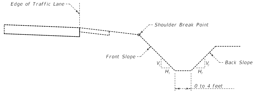
Figure 4.2.14 Roadside Ditches – Bottom Width 0 to 4 feet
