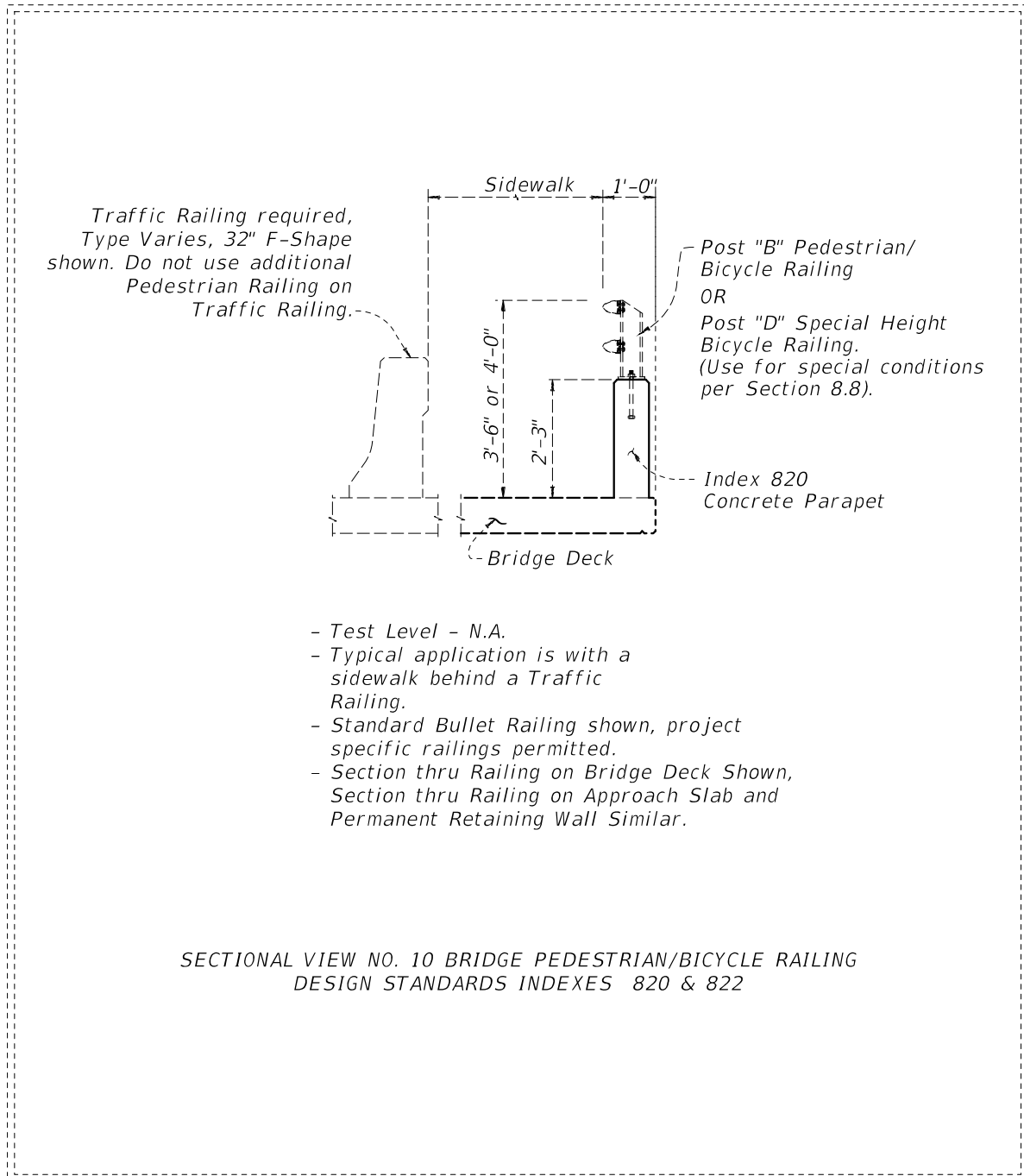
Figure 4.4.5 Bridge Railing – Pedestrian/Bicycle Railing (Index 820)
