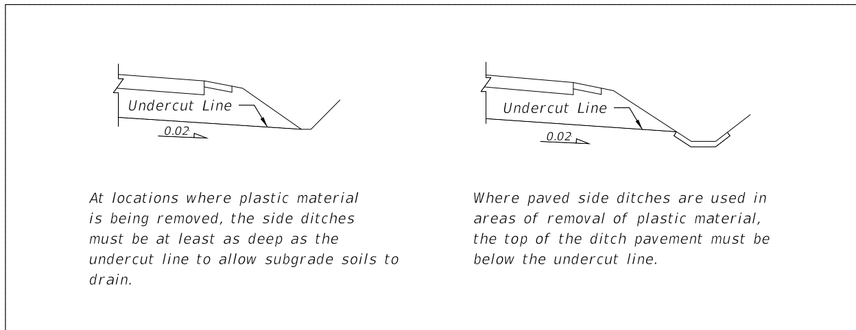
Figure 3.5.2 Undercut Detail of Plastic Material with Relation to Side Ditches
