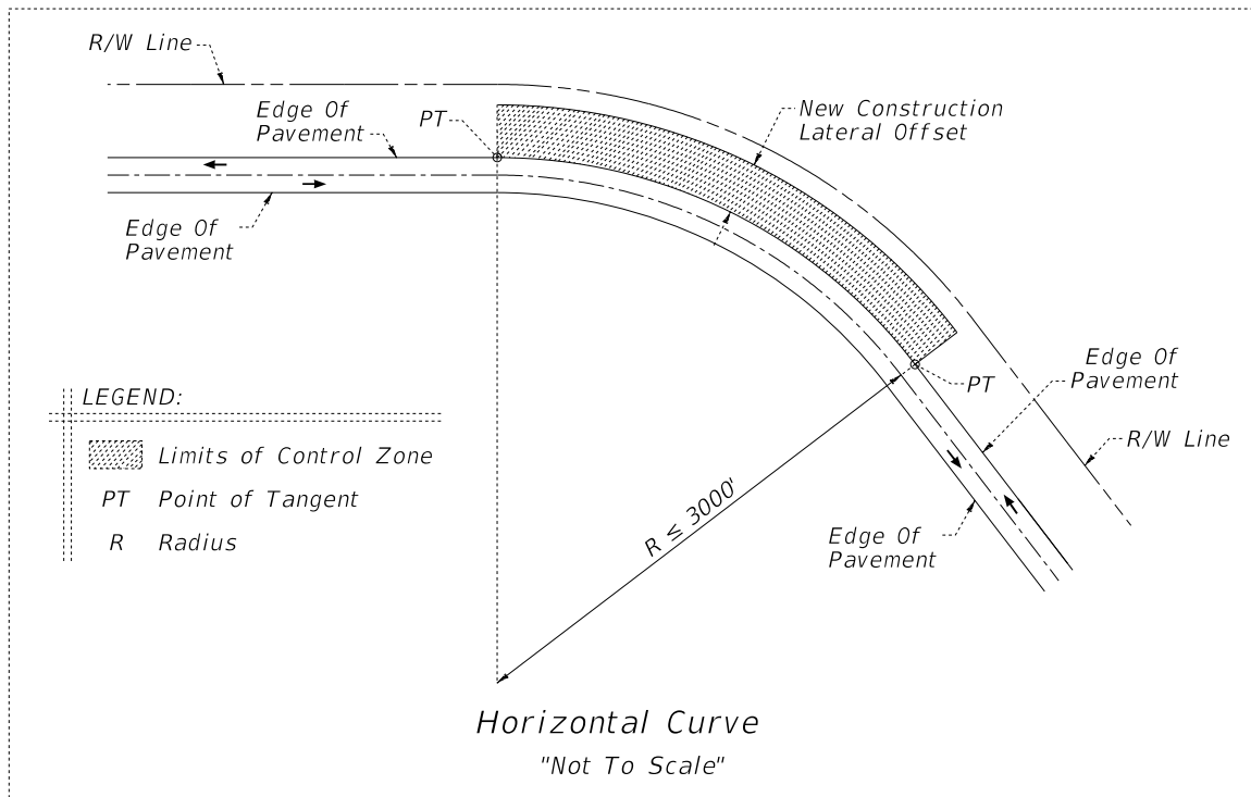
Figure 4.2.12 Horizontal Curve
