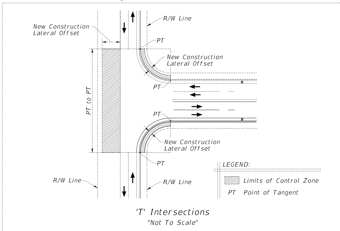
Figure 4.2.5 'T' Intersection
