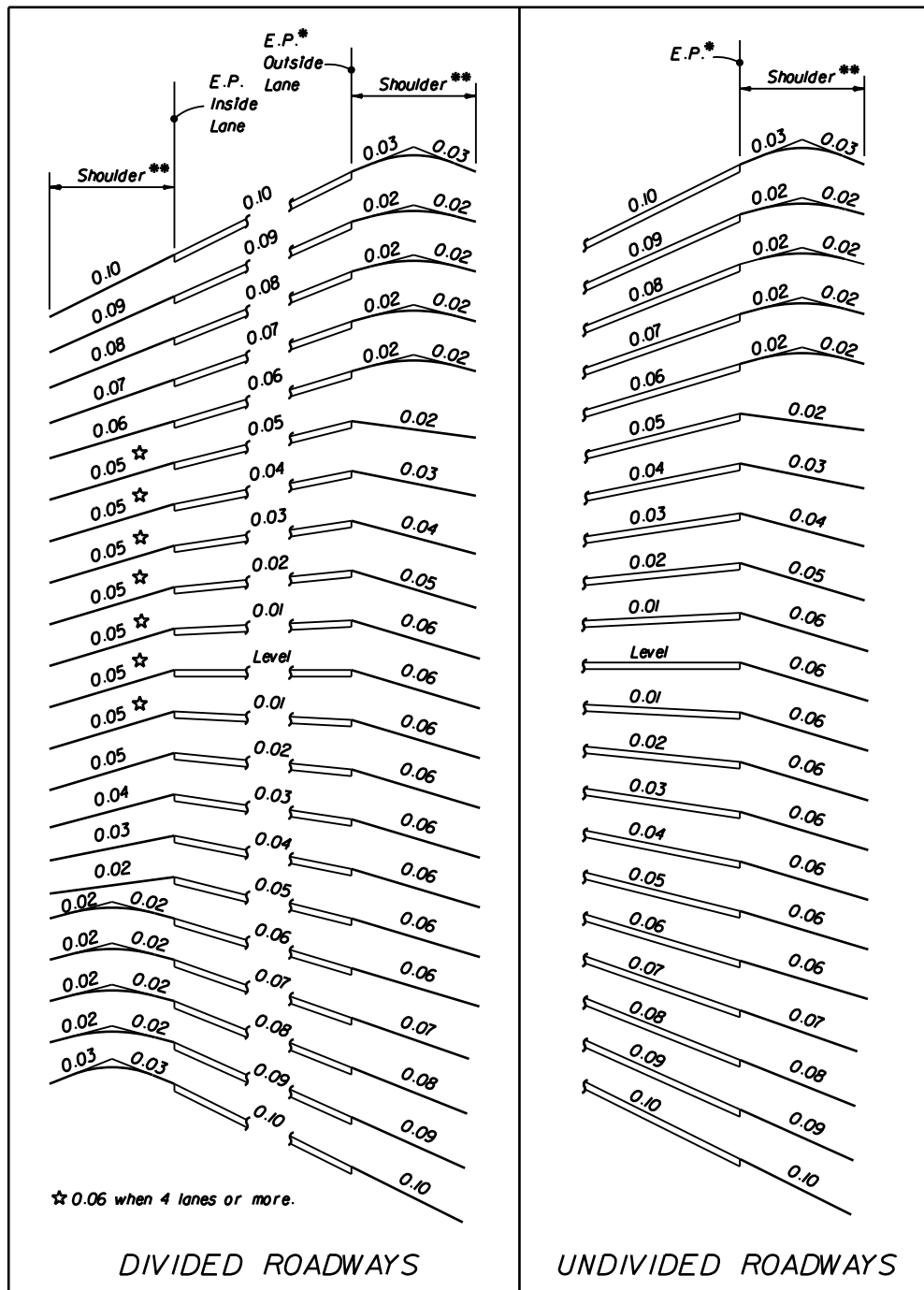
Figure 2.3.1.A Shoulder Superelevation
