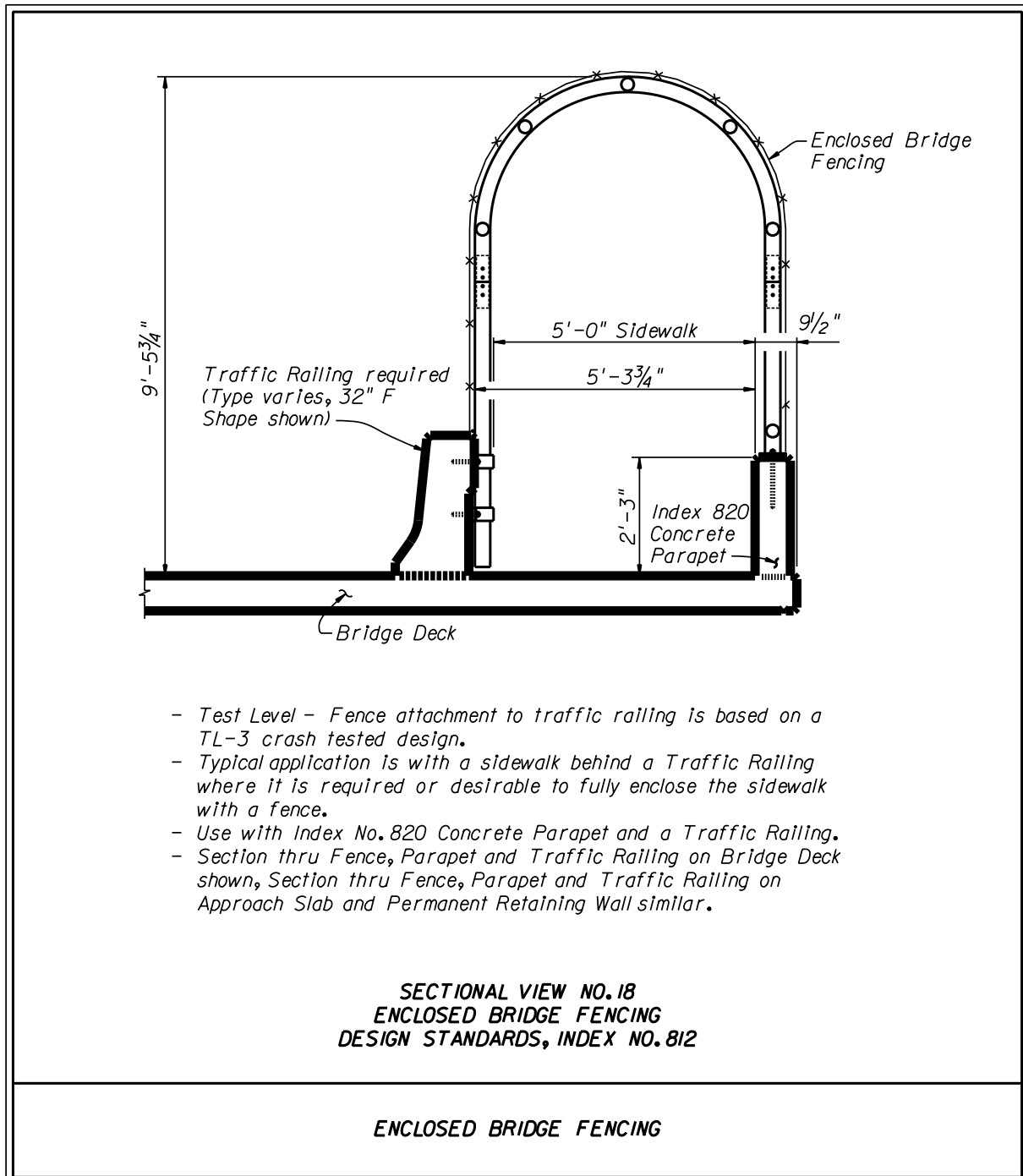
Figure 2.12.12 Enclosed Bridge Fencing for Pedestrian Railing
