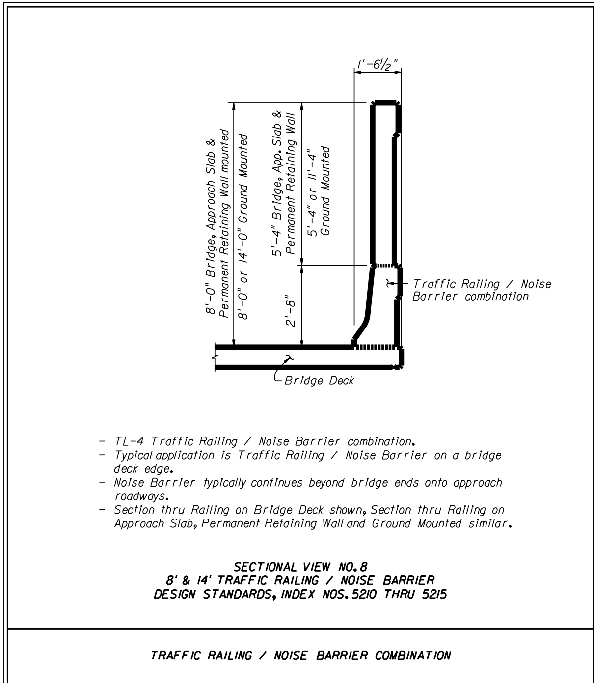
Figure 2.12.4 Bridge Traffic Railings – Noise Barrier Combination
