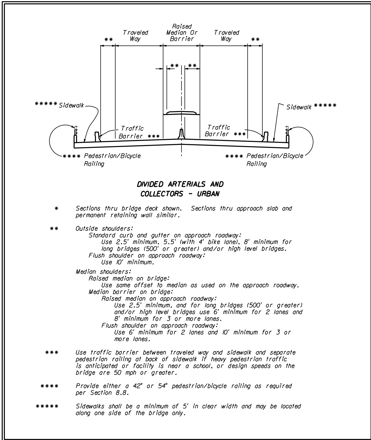
Figure 2.0.4 Bridge Section *
