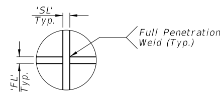
DETAIL 'P'
