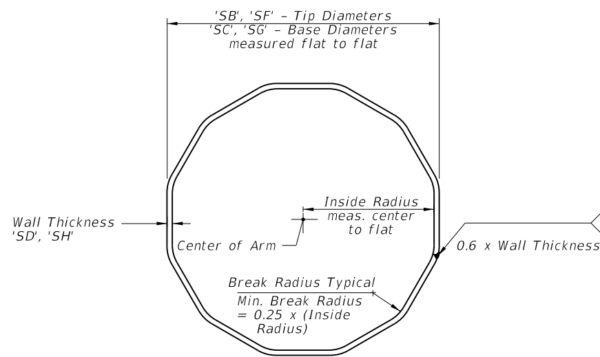
SECTION M-M
