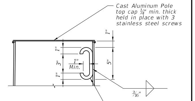
POLE TOP CUT-AWAY (Option 'b')
