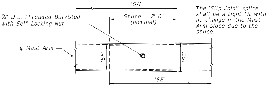
Arm Splice Detail
