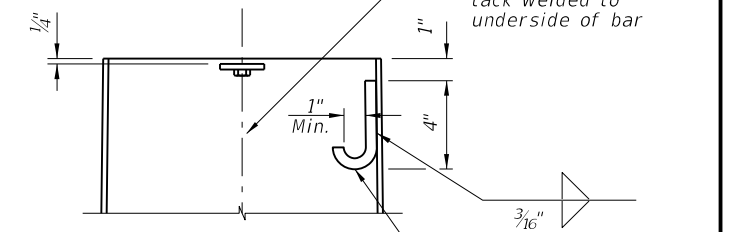
POLE TOP CUT-AWAY (Option 'a')
