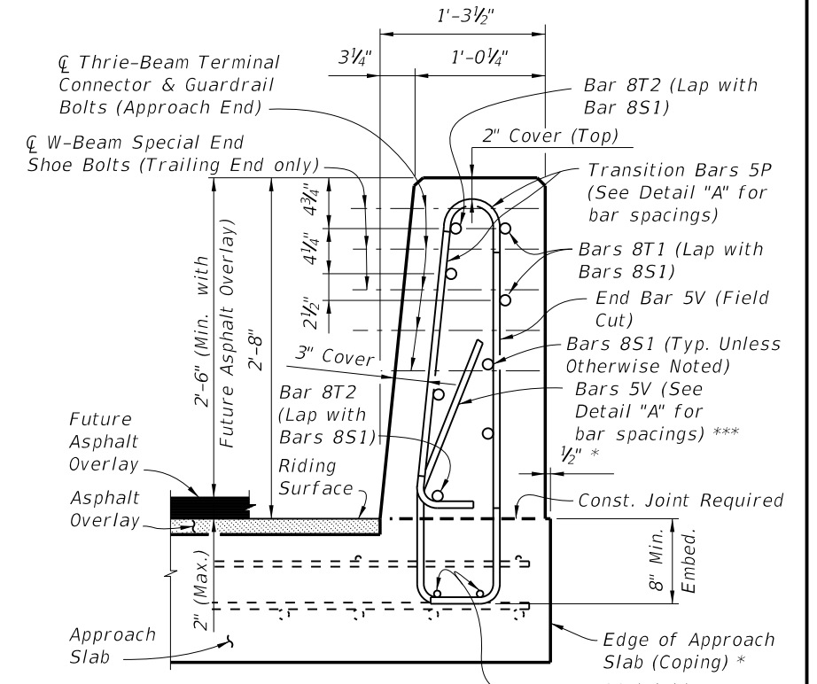
VIEW B-B (Section thru Approach Slab shown, Section thru Retaining Walls similar)
