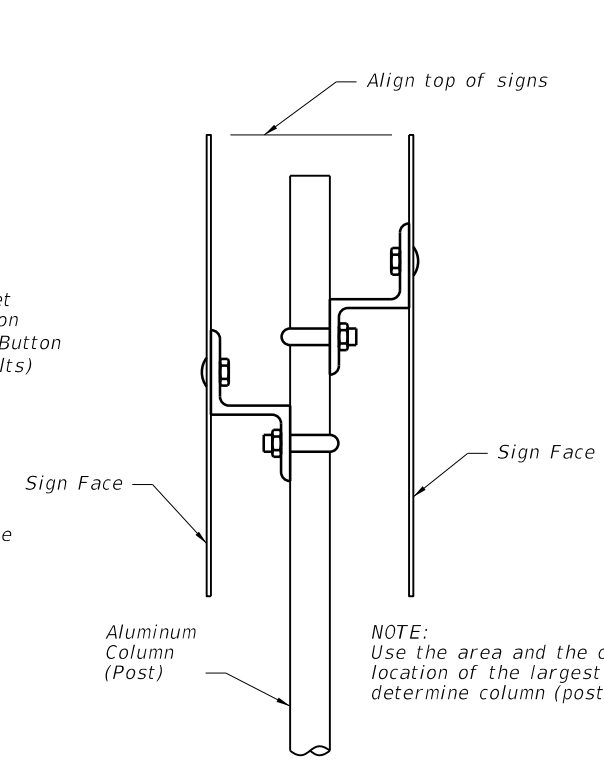
SIGNS BACK-TO-BACK
