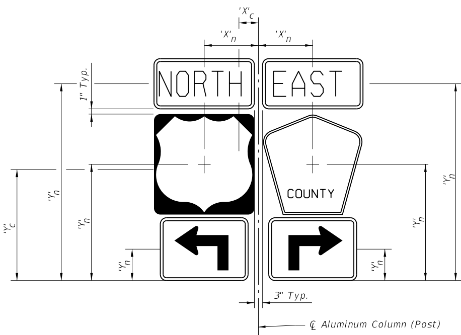
SIGN CLUSTER
