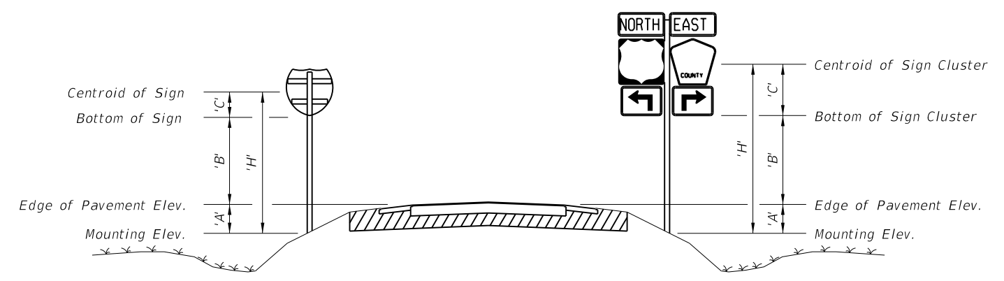
TYPICAL SECTION
