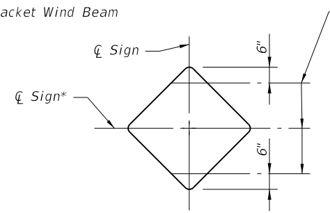
DIAMOND
