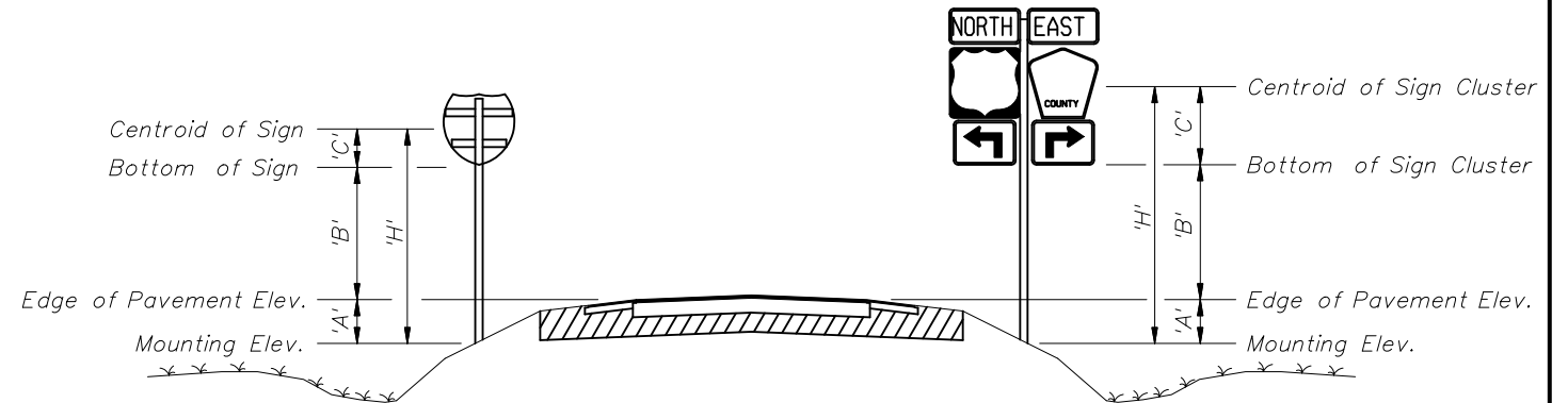
TYPICAL SECTION
