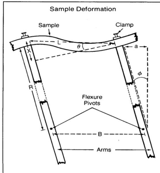
Figure 4.6 Sample Deformation
