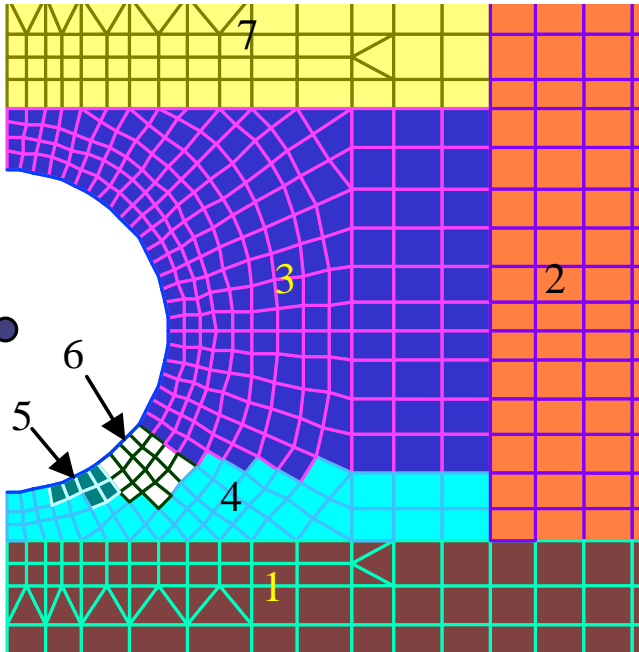
Fig. 1.2 – Soil zones
