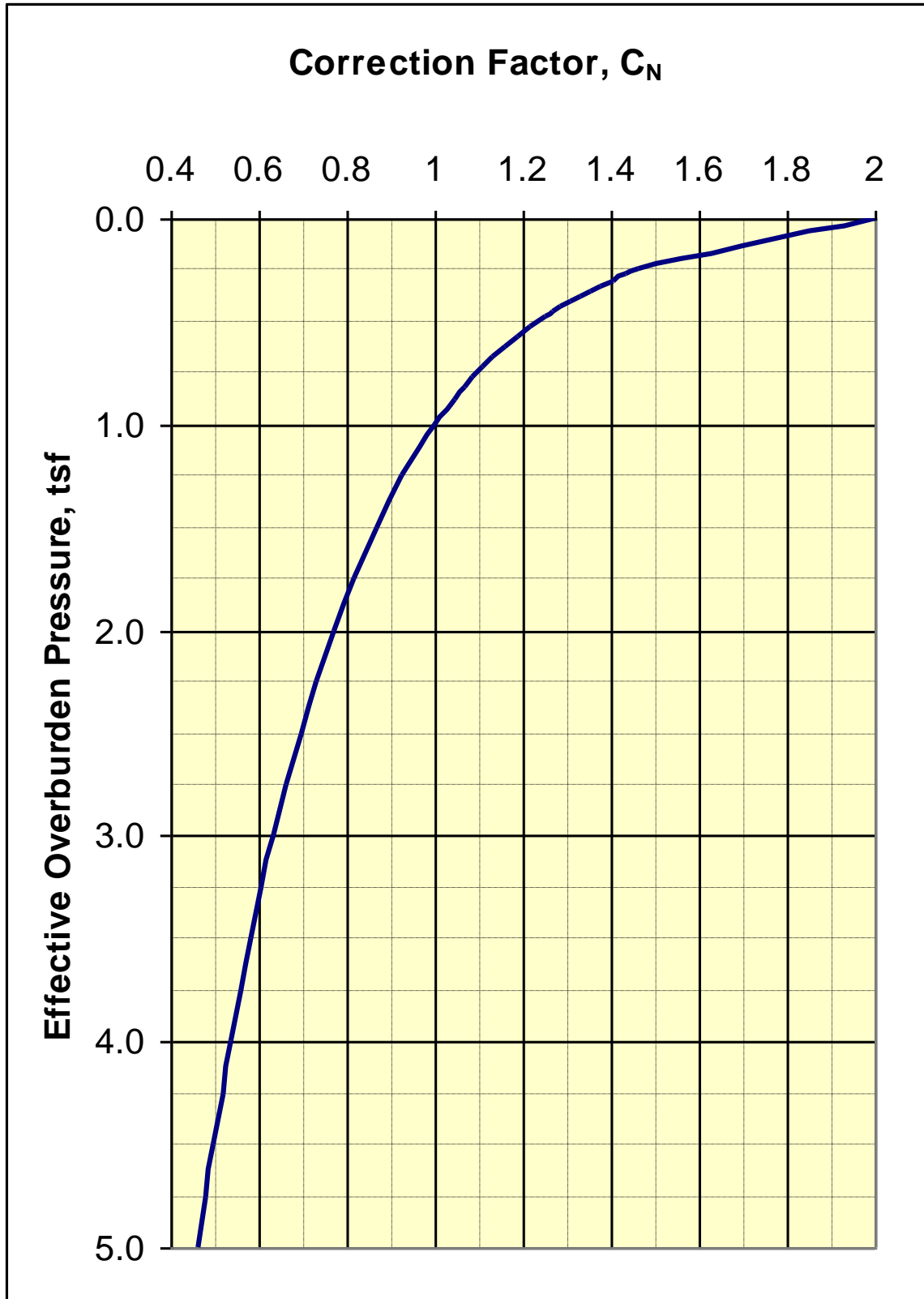
Figure 18 - C N vs. Effective Overburden Pressure (After Peck, 1974)
