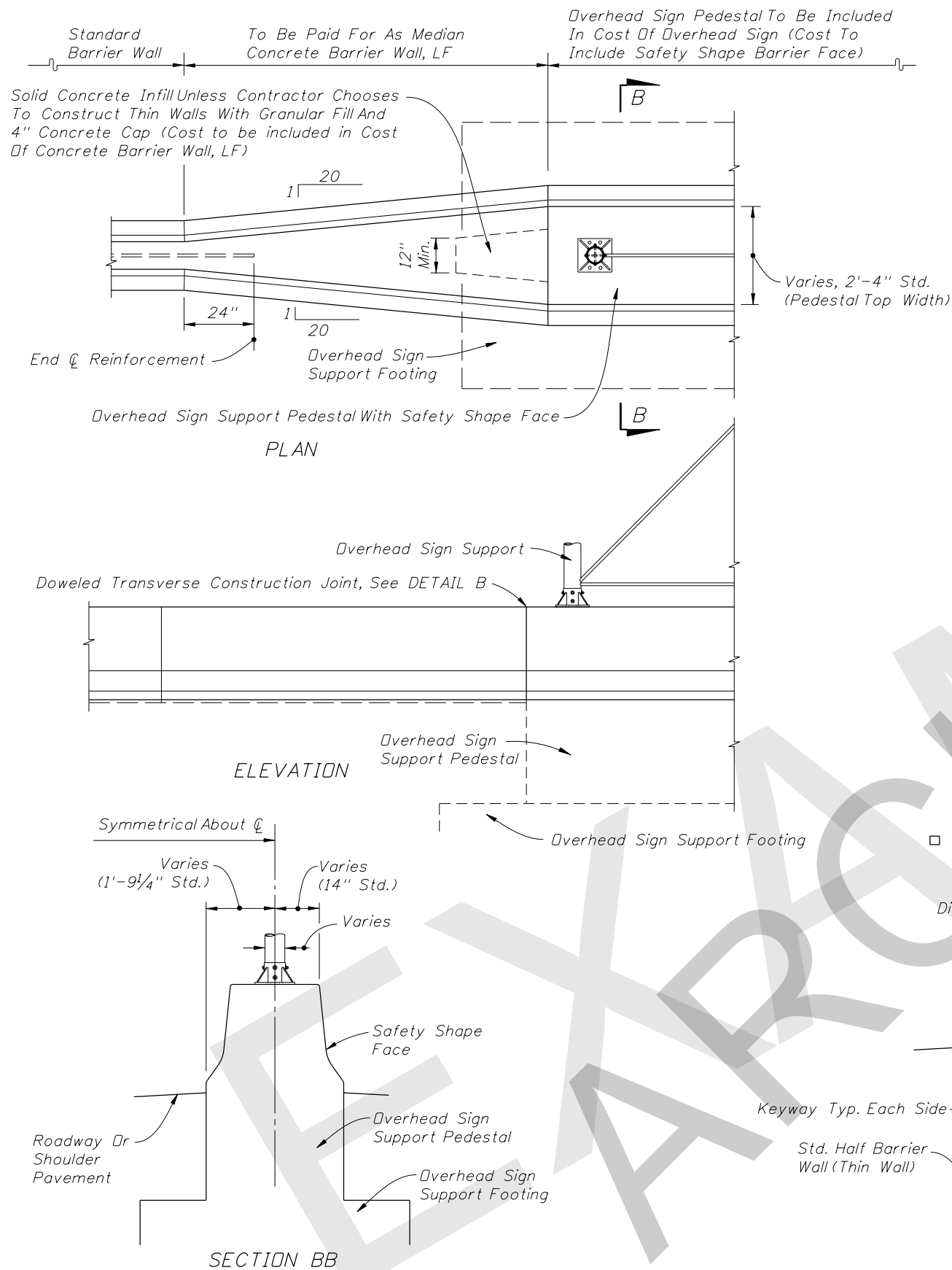
COMBINATION BARRIER AND SIGN PEDESTAL CONCRETE MEDIAN BARRIER WALL TRANSITIONS AT OVERHEAD SIGN SUPPORTS
