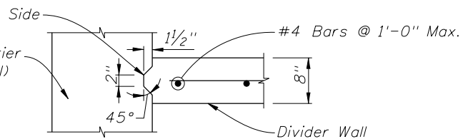
SECTION FF
