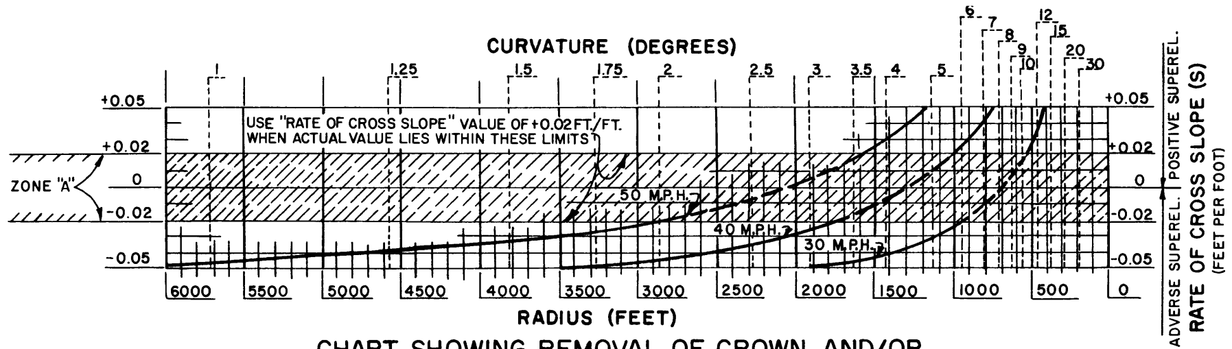
CHART SHOWING REMOVAL OF CROWN AND/OR SUPERELEVATION NECESSARY FOR CURVATURE AT VARIOUS DESIGN SPEEDS
