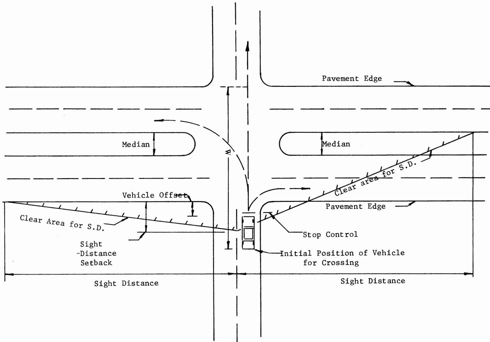
INTERSECTION CONFIGURATION
