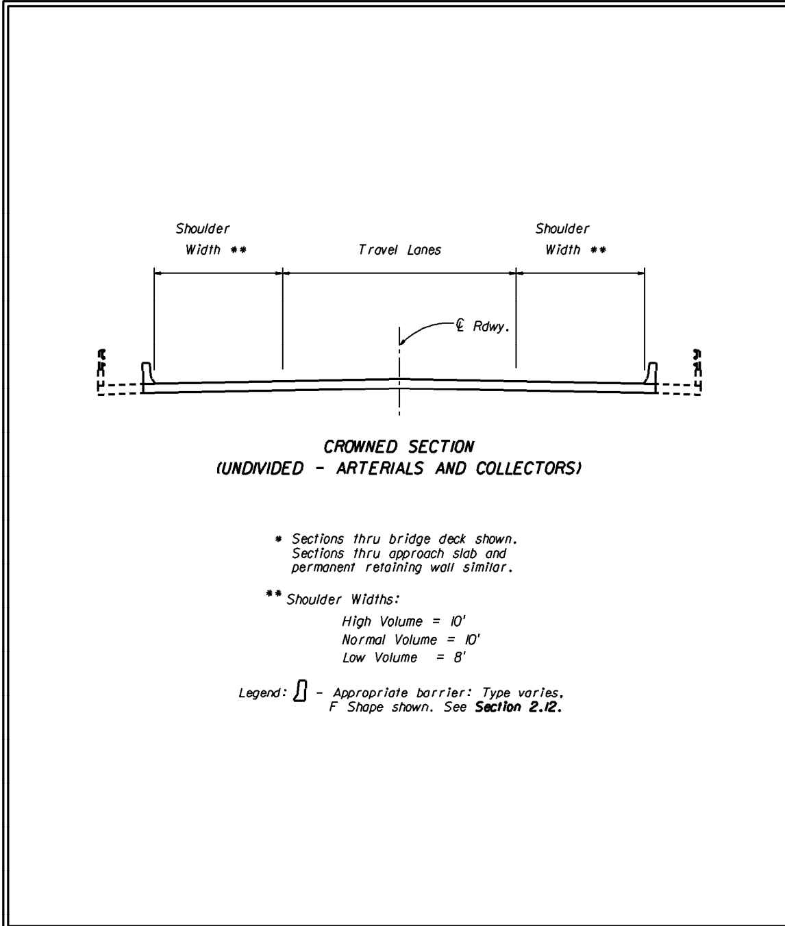
Figure 2.0.2 Bridge Section *
