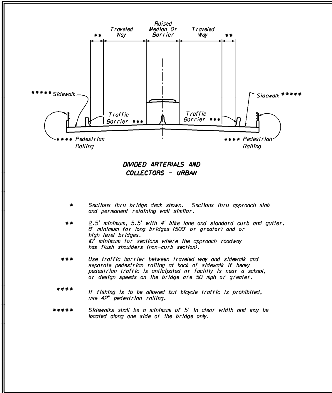
Figure 2.0.4 Bridge Section *
