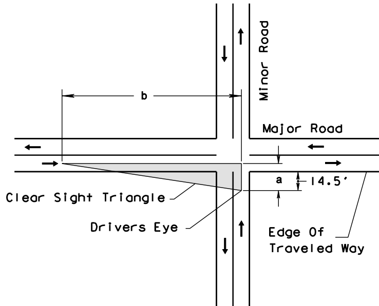
FIGURE 3 - 7 DEPARTURE SIGHT TRIANGLE TRAFFIC APPROACHING FROM LEFT OR RIGHT
