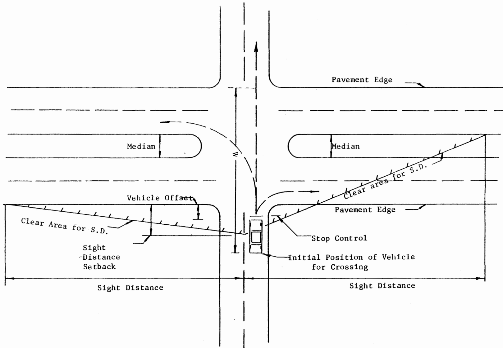
INTERSECTION CONFIGURATION
