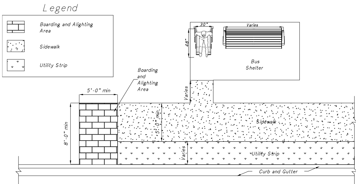
Figure 13 – 3 Bus Shelter Location
