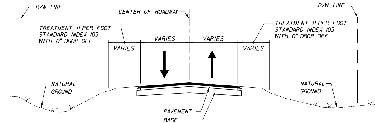
Figure 5 – 1 Two Lane Road w With Safety Edge
