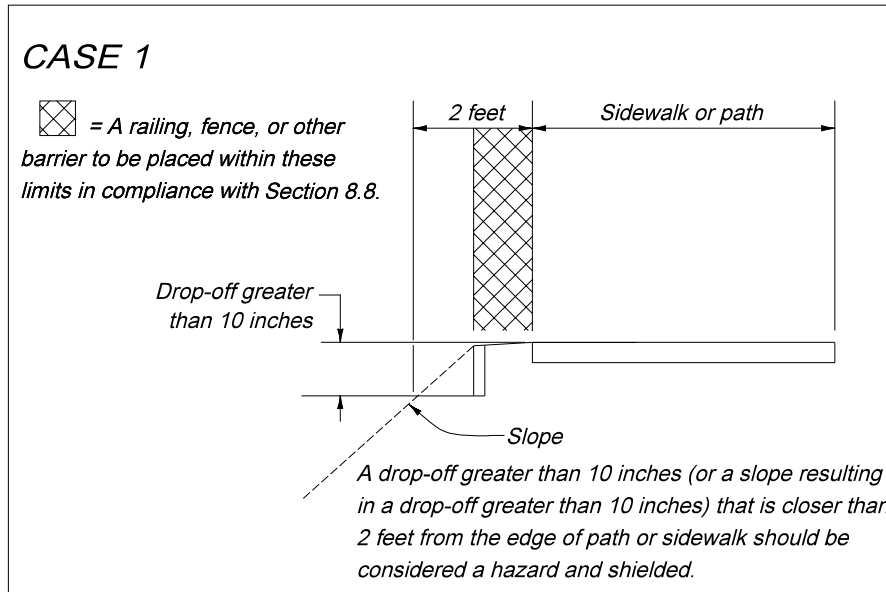
Figure 8 – 45 Drop-Off Hazards for Pedestrians and Bicyclists
