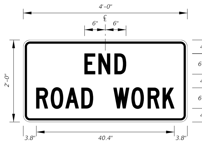
G20-2 2' X 4' 1.5" Radii 3/4" Border
