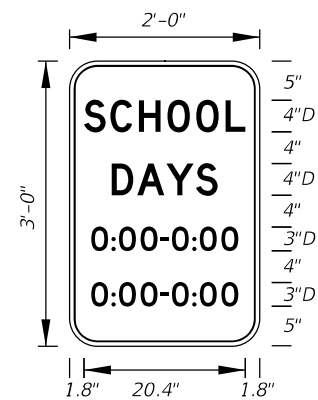
FTP-30-06 2'-0" X 3'-0" 3" Radii 5/8" Border White Background Black Legend and Border
