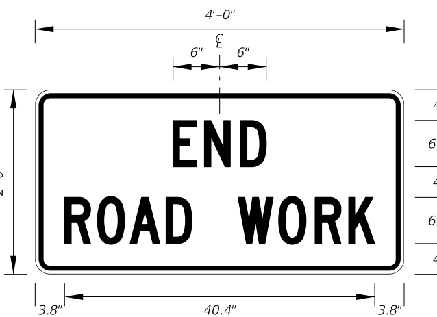
G20-2 2' X 4' 1.5" Radii 3/4" Border Orange Background Black Legend and Border
