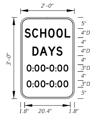
FTP-30-06 2'-0" X 3'-0" 3" Radii \frac{5}{8} " Border White Background Black Legend and Border
