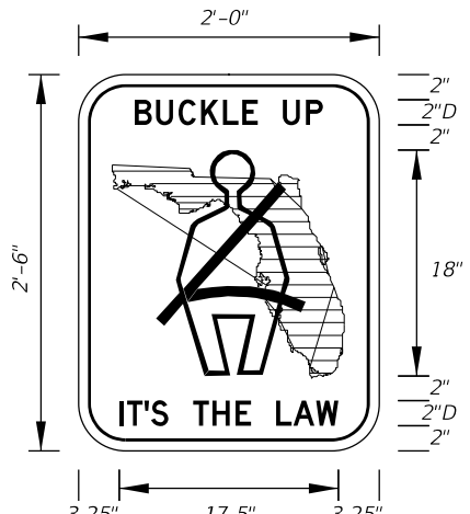
FTP-47-06 2' X 2'-6" 3" Radii 5/8" Border 2" Series D Legend White Background Black Legend, Border and Man Belt Symbol Florida Shield Green
