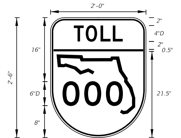
FTP-81-06 2' X 2'-6" 3" Radii 3/4" Border 4" and 6" Series D Legend Top Yellow Background with White Legend and Black Border Bottom White Background with Black Legend and Border
