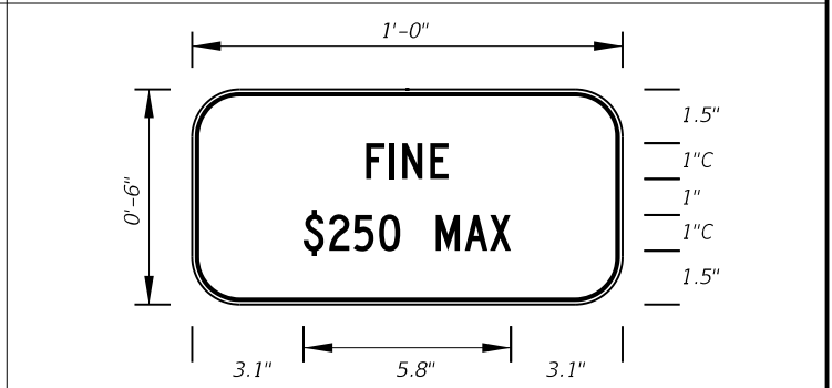
FTP-22-06 1' X 6" 1" Radii 3/8" Border 1" Series C Legend White Background Black Legend and Border
