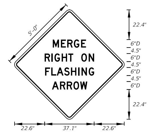
M0T-8-06 5' X 5' 2" Radii 3/4" Border 6" Series D Legend Orange Background Black Legend and Border
