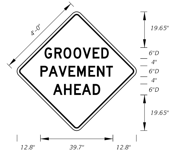
M0T-15-06 4' X 4' 2" Radii 3/4" Border
