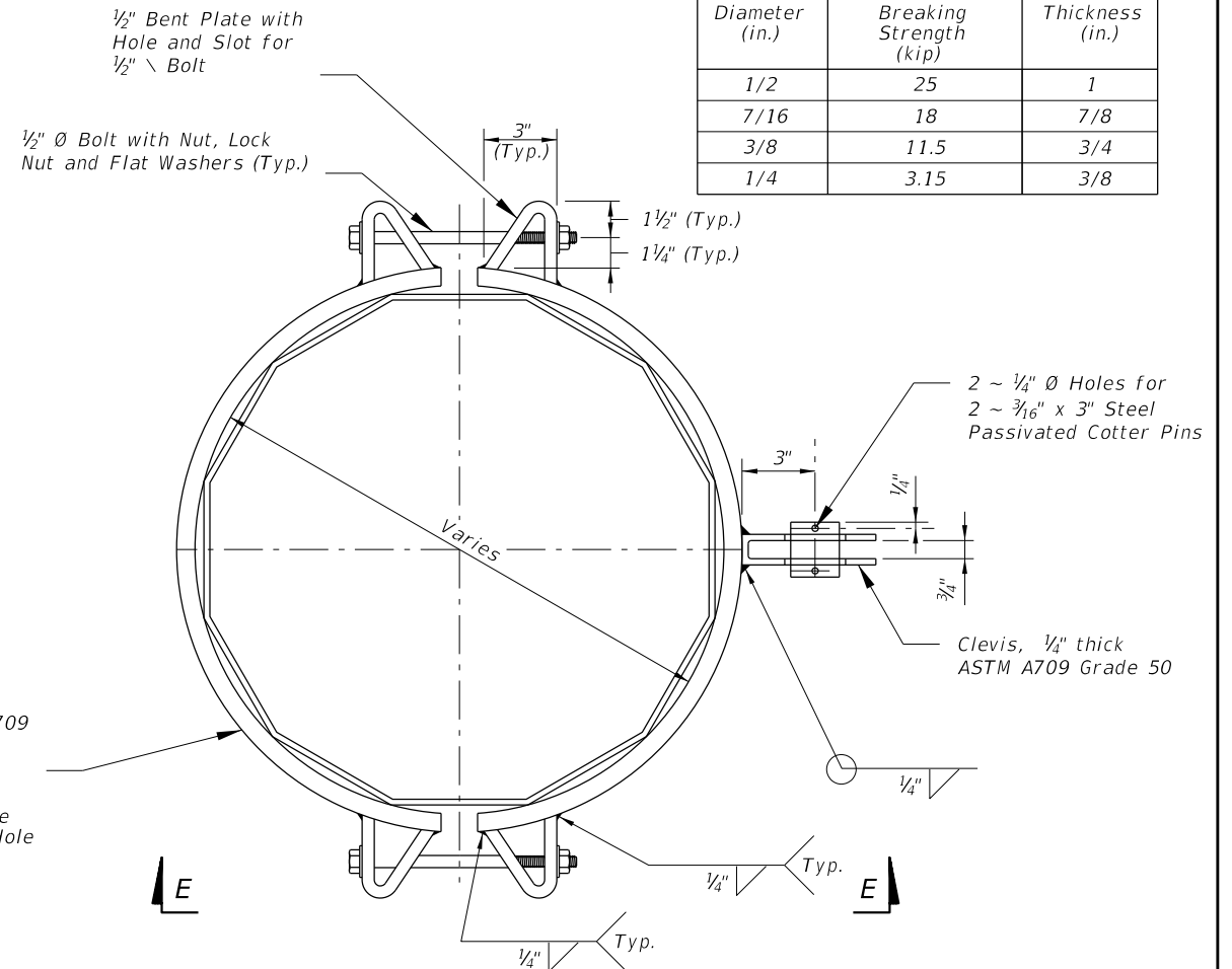
CATENARY AND MESSENGER WIRE CLAMPS
