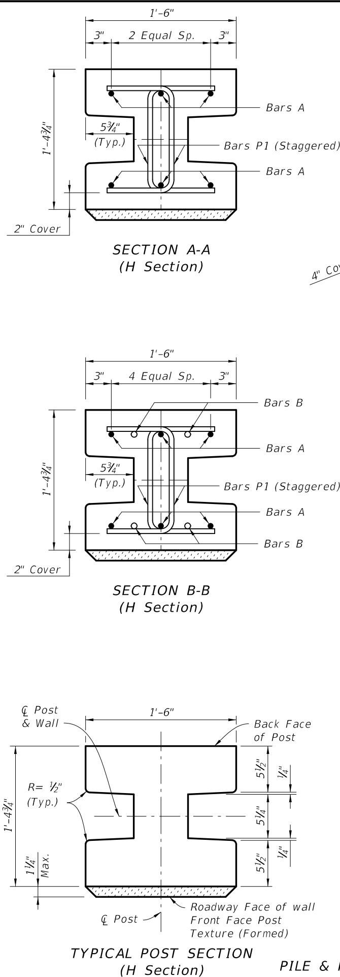
GROUND MOUNTED POST REINFORCEMENT (Prior to placement in augered hole)
