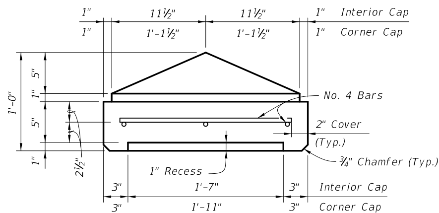
SECTION C-C
