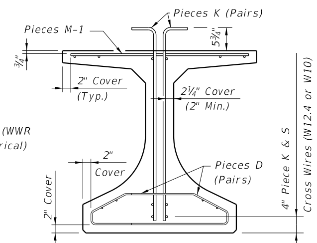
PARTIAL BEAM END VIEW (Conventional Reinforcing Bars A, C, Y and Strands not Shown for Clarity)
