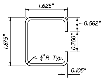
THINWALL
