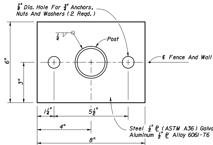
TOP VIEW TWO ANCHOR OPTION
