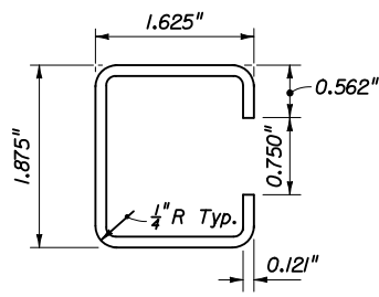
STANDARD WALL
