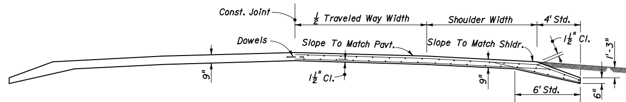
SECTION AA
