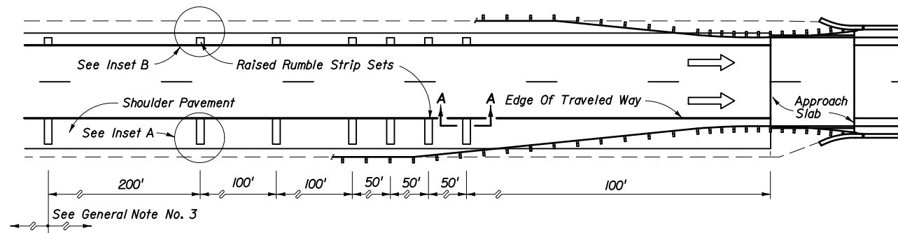
PLAN • ONE-WAY
