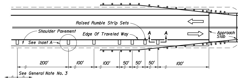
PLAN • TWO-WAY
