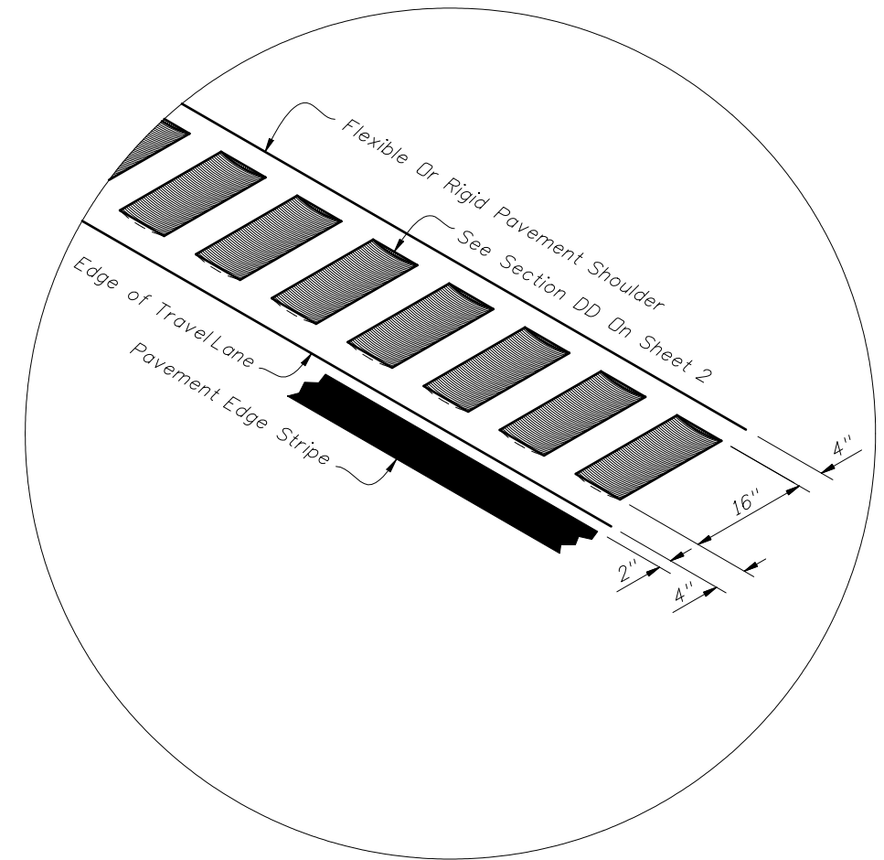
ISOMETRIC - LONGITUDINAL CUT (RIGID PAVEMENT)
