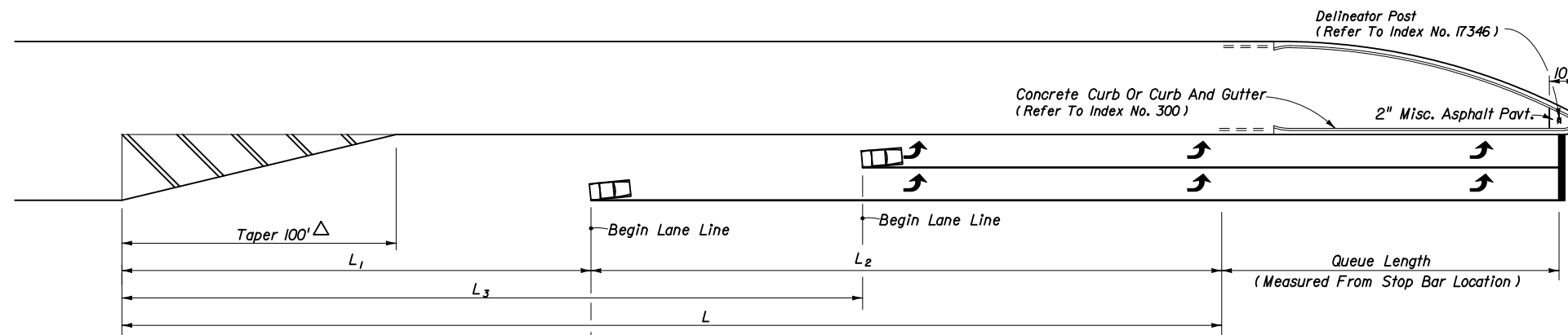
FLUSH AND/OR CURBED SEPARATION
