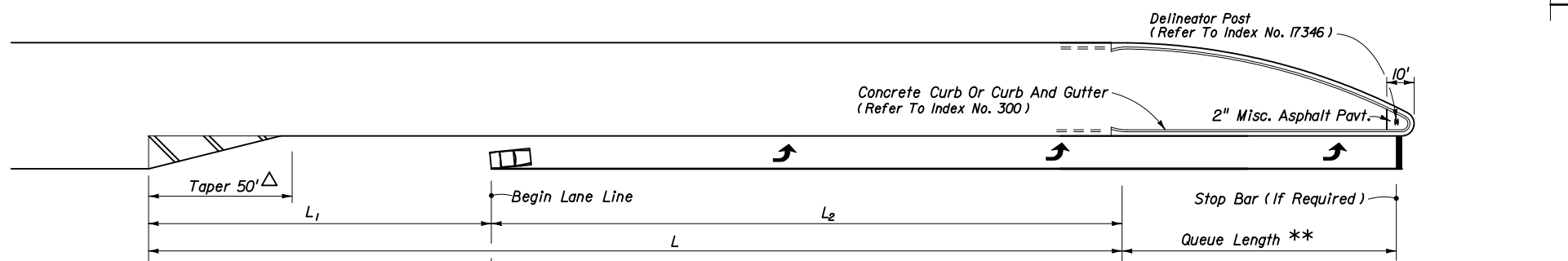
FLUSH AND/OR CURBED SEPARATION
