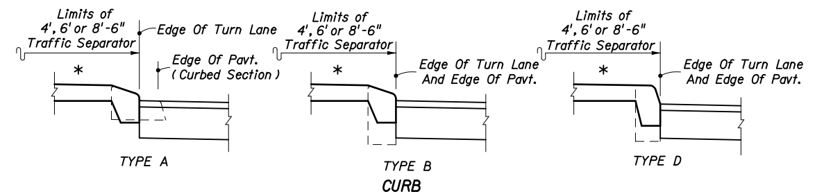
CURB AND GUTTER
