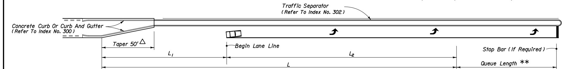
RAISED SEPARATION SINGLE LEFT TURNS
