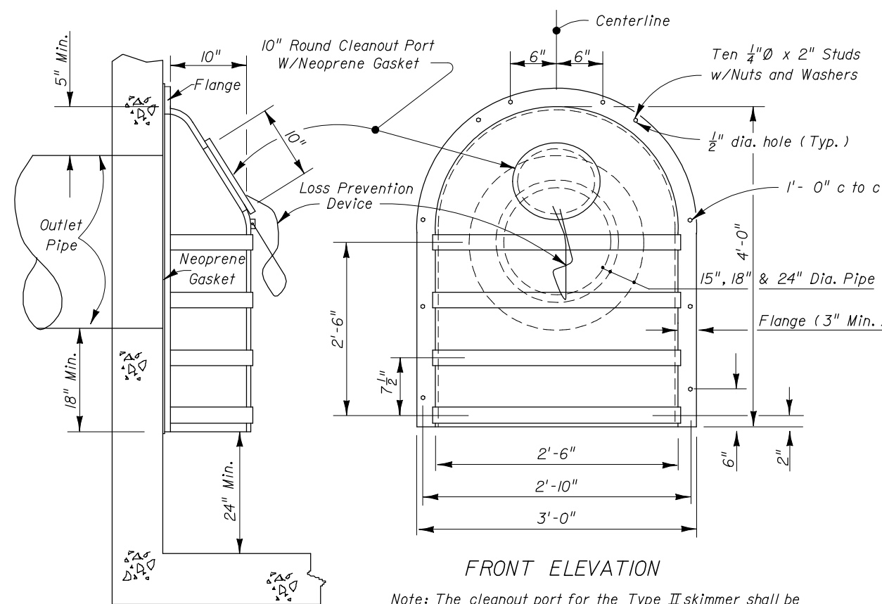
TYPE II SKIMMER
