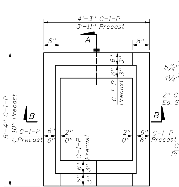
PLAN (CAST-IN-PLACE INLET WITHOUT GRATE SHOWN, PRECAST INLET SIMILAR)
