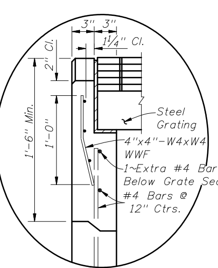
INSET A (PRECAST OPTION)
