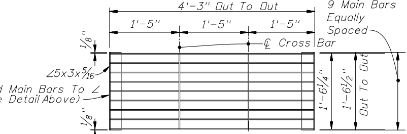
TOP VIEWS Main Bars 5"x1/4" (Notched For Cross Bars) Cross Bars 1 3/4"x1/4" (3/16" Continuous Weld At Main Bar Notches) Main Bars and Cross Bars Flush On Top
