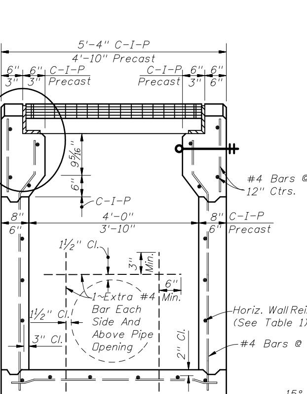
SECTION AA (CAST-IN-PLACE INLET SHOWN, PRECAST INLET SIMILAR)
