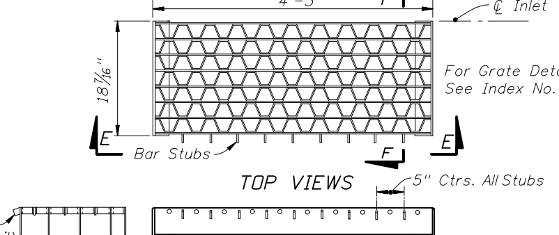
SECTION EE STEEL GRATE
