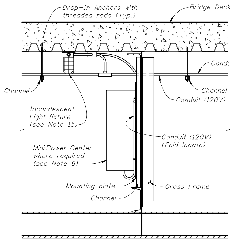
SECTION C-C
