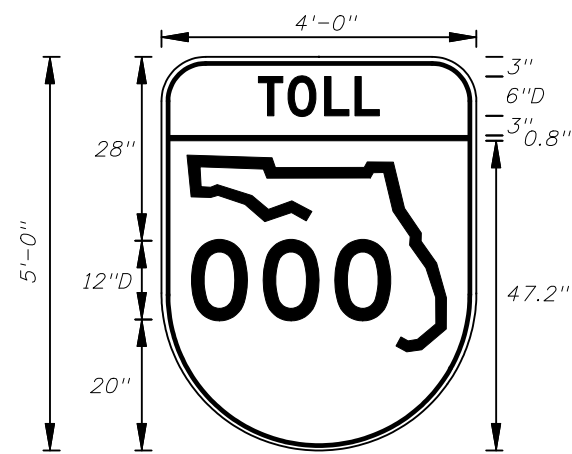
FTP-79-06 4' X 5' 6" Radii \frac{3}{4} " Border 6" and 12" Series D Legend Top Green Background with White Legend and Black Border Bottom White Background with Black Legend and Border
