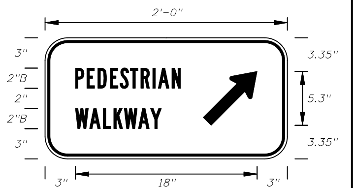
MDT-12-06 2' X 1' 2" Radii 3/4" Border
