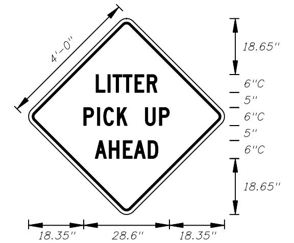
MDT-4-06 4' X 4' 2" Radii 3/4" Border
