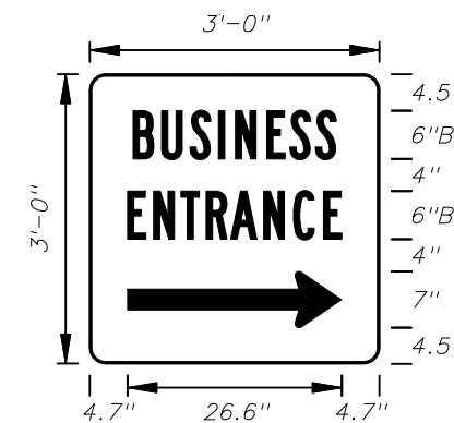
MDT-11-06 3' X 3' 2" Radii 3/4" Border
