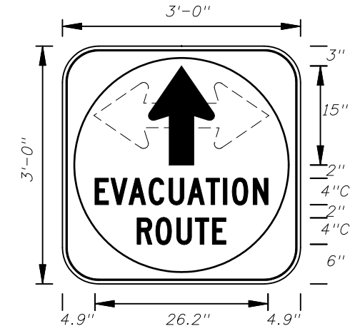
FTP-77-06 3' X 3' 5" Radii \frac{3}{4} " Border 4" Series C Legend White Background with Blue Circle Background White Legend and Black Border
