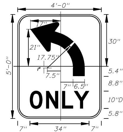
FTP-54-06 4' X 5' 6" Radii \frac{3}{4} " Border 10" Series D Legend White Background Black Legend and Border
