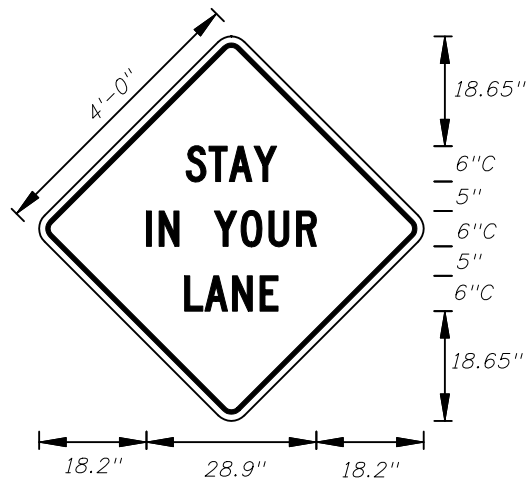
MDT-1-06 4' X 4' 2" Radii 3/4" Border
