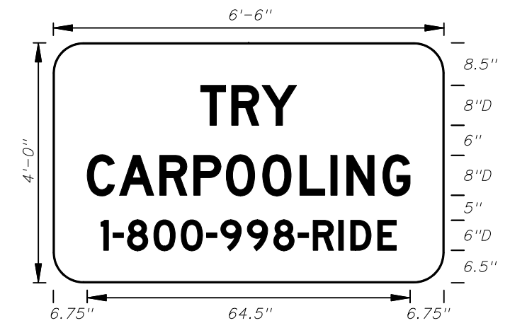
FTP-56-06 6'-6" X 4' 6" Radii \frac{3}{4} " Border 8" and 6" Series D Legend Blue Background White Legend and Border
