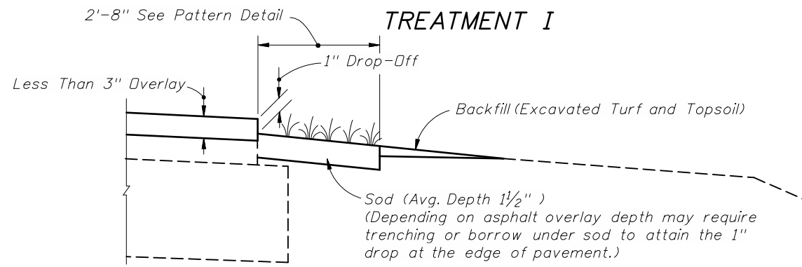
COMPLETED SHOULDER
