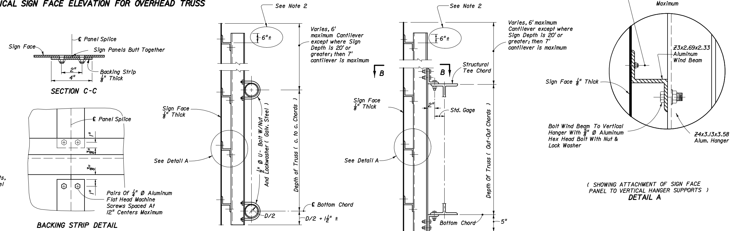
TYPICAL DETAILS OF SIGN & TRUSS CONNECTION ( LIGHTING NOT SHOWN )
